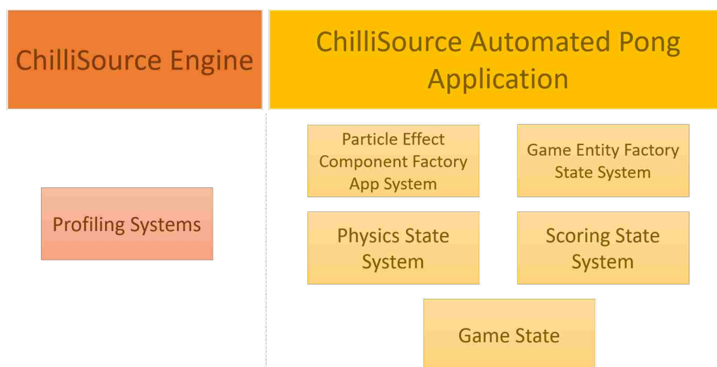
Figure 3.2: The basic architecture of the automated pong game. This shows CSAPong having a Particle Effect Component Factory App System , a Game Entity State System , a Physics State System , a Scoring State System , and the Game State itself. Although the entirety of the ChilliSource engine is used in CSAPong, this graph highlights the custom Profiling Systems within ChilliSource that I created for the purposes of instrumenting Particle Effect Components .
