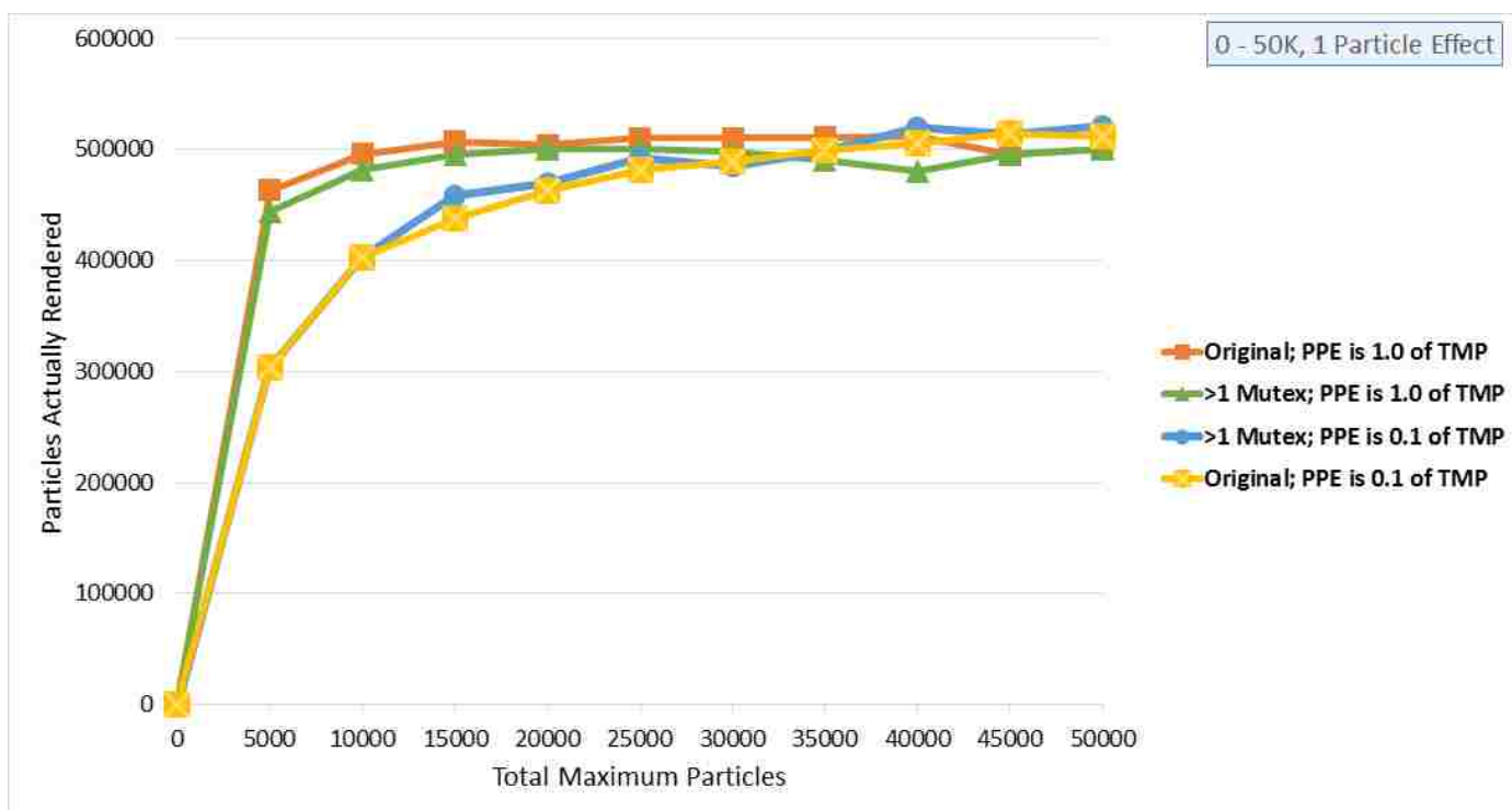
Figure 4.7 A graph showing particles actually rendered over total maximum particles for a single particle effect. This shows that changing Concurrent Particle Data to use multiple mutexes also does not impact the number of times that particles are rendered. As in Figure 4.6, the > 1 Mutex data series is almost the same as the ones for the data series without any changes to the source code (i.e. the Original data series).
