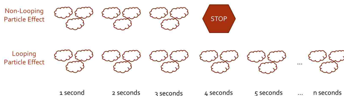
Figure 5.21: Demonstrates the difference between looping and non-looping particle effects that both have a duration of 3 seconds. Each particle effect emits once every second, but the non-looping particle effect will stop emitting after 3 seconds have elapsed. It's important to note that, although the non-looping particle effect has stopped emitting, ChiliSource will continue to render any active particles on the screen from previous emissions. The engine will only clean up the particle effect if there are no longer any active particles on the screen.
