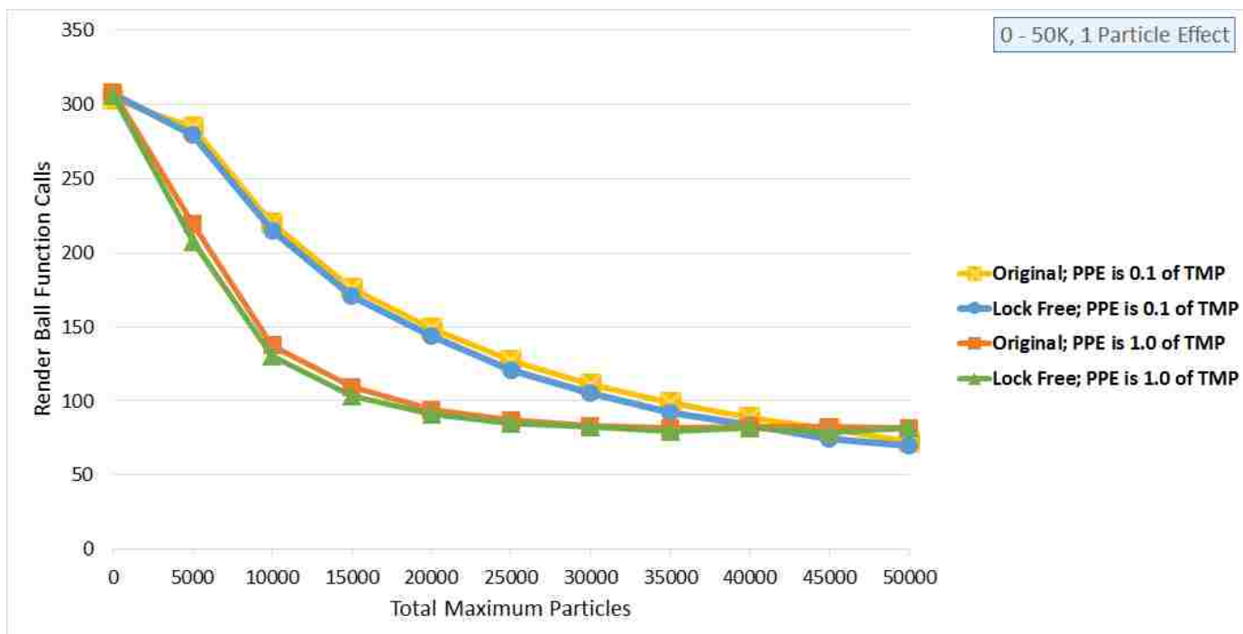
Figure 4.11 A graph showing render ball function calls over total maximum particles for a single particle effect. This shows that changing Concurrent Particle Data to use a lock free data structure does not impact the number of times that the ball is rendered. The multiple-burst and single-burst (0.1 and 1.0 TMP, respectively) scenarios for the Lock Free data series are almost the same as the ones for the data series without any changes to the source code (i.e. the Original data series).
